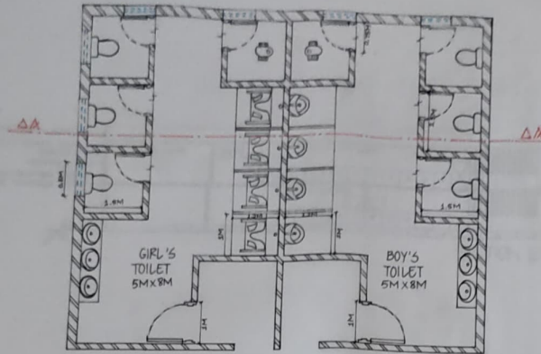
DETAIL OF TOILET [PLAN]
