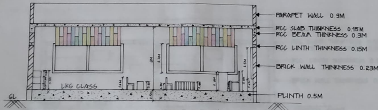
SECTION @ ΔΔ'
